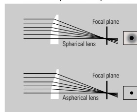
Spherical aberration of spherical lenses and corrected images using aspherical lenses.
